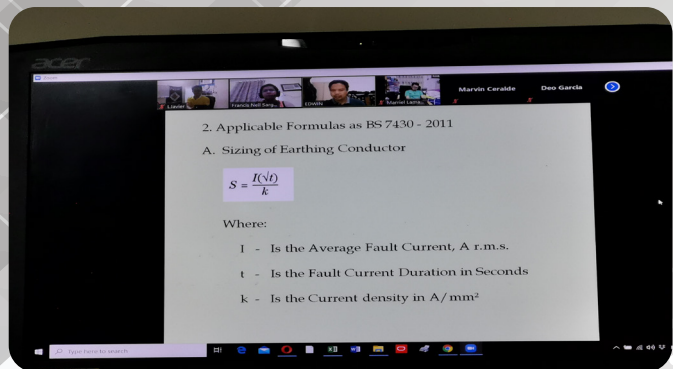
Engr. Edwin Cayabyab discussing Grounding Calculation on March 24, 2020.
